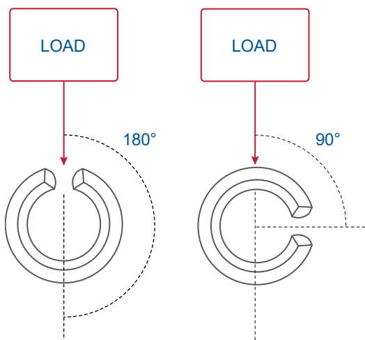
Figure 4 Orientation of the slot affects shear strength in Slotted Spring Pins by approximately 5%
