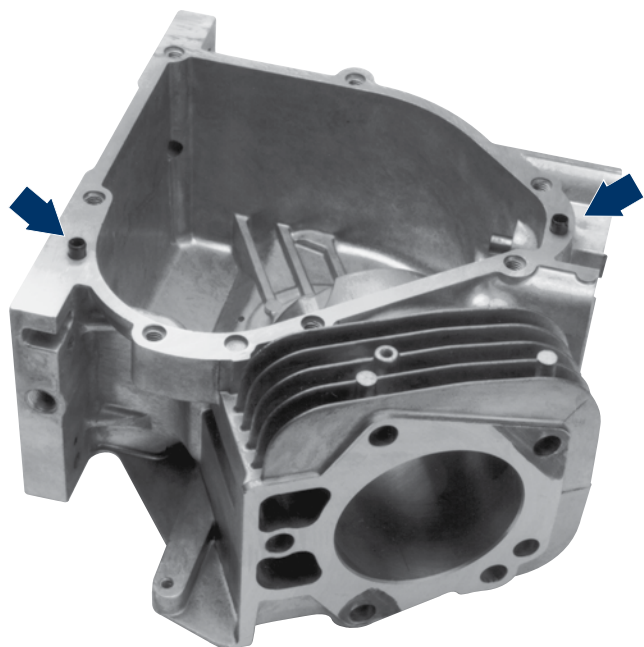
ENGINE HOUSING
